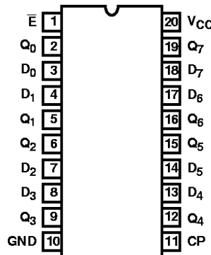
CD74HC377, CD74HCT377 (PDIP, SOIC) TOP VIEW
