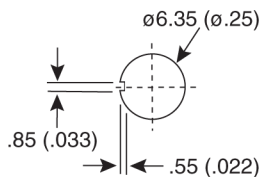
PANEL MOUNTING
