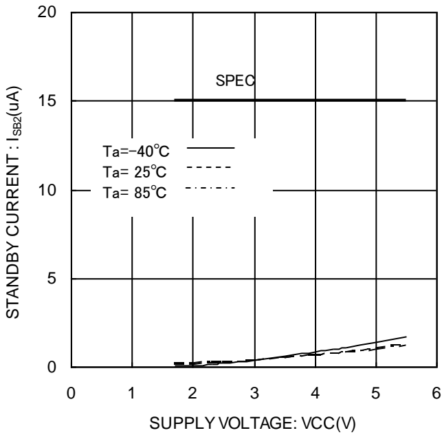
Figure 20. Standby current I_{SBZ}(CS=0V, ORG=0V)
