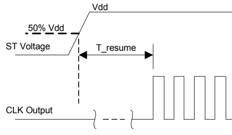
Figure 5. Standby Resume Timing (ST Mode Only)
