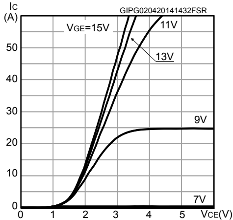
Figure 3. Output characteristics ( T_J = 25 °C)
