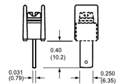
09 0.250" QC short
