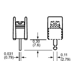
06 Handwired
