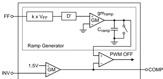
Figure 8. Ramp Generator
