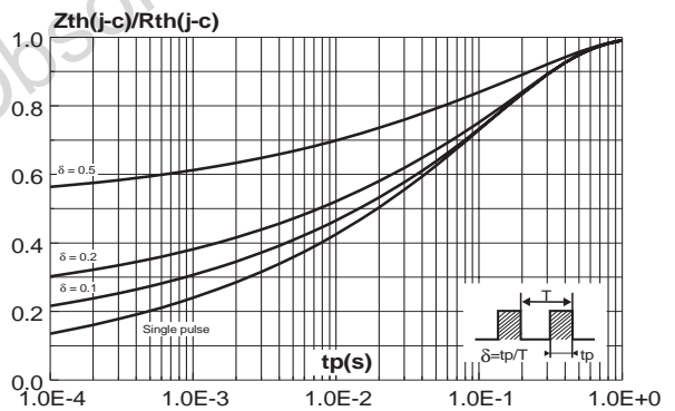
Fig. 6: Relative variation of thermal transient impedance to case versus pulse duration.
