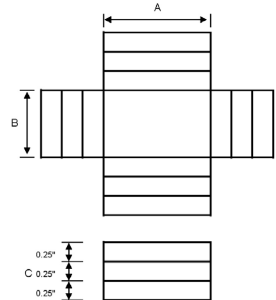
Each 0.25" section can be easily broken away to create shield heights of 0.25", 0.50" or 0.75"
