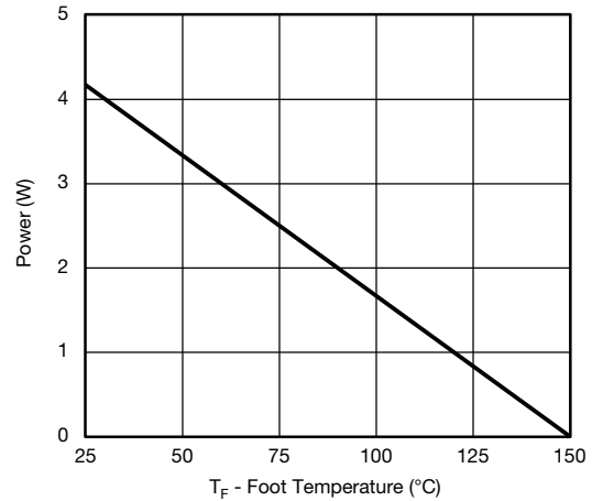
Power, Junction-to-Foot
