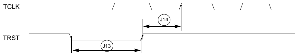
Figure 27. \overline{\text{TRST}} Timing
