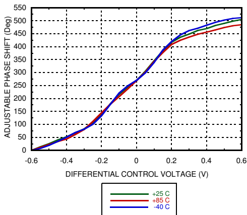
Phase Shift vs. Temperature [1][2][3][4]
