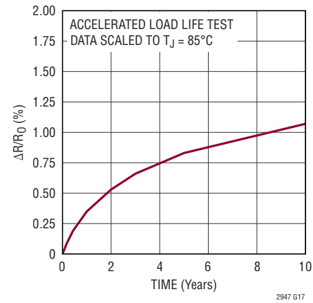
Sense Resistor Stability
