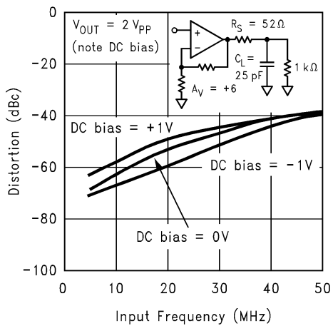
2nd Harmonic Distortion C_L = 25 pF
