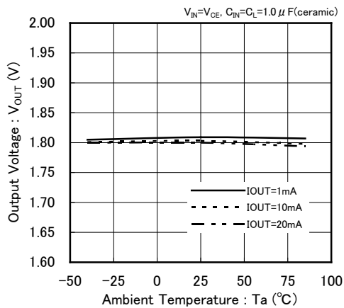
XC6701A/B/D 182
