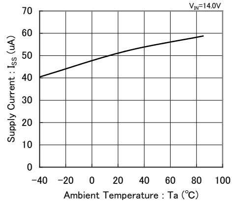
XC6701A/B/D J02
