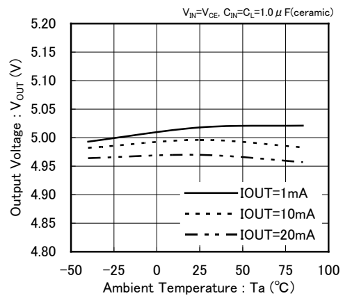
XC6701A/B/D 502
