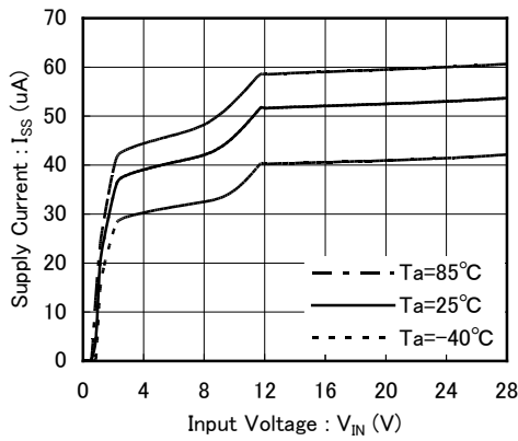
XC6701A/B/D J02
