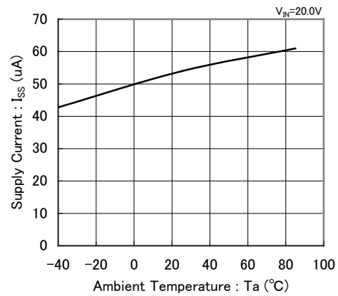
XC6701A/B/D J02
