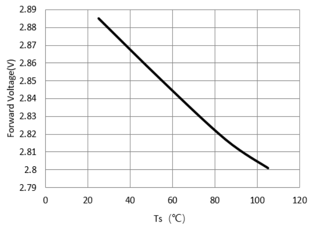
Temperature vs. Forward Voltage (I f =120mA)
