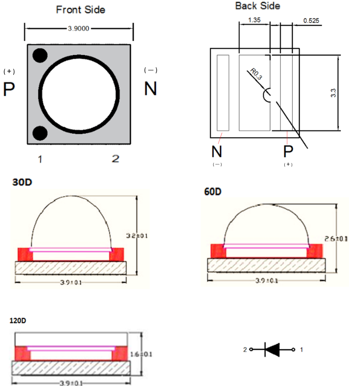
Figure 2. IN-C39ATKU1 / IN-C39BTKU1 / IN-C39CTKU1 Package Dimension
