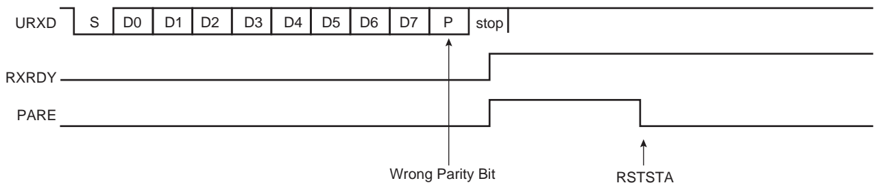
Figure 30-7. Parity Error
