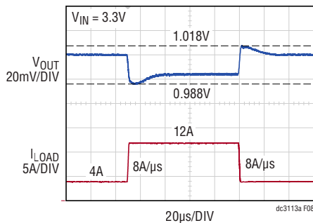
Figure 8. Load Step Response
