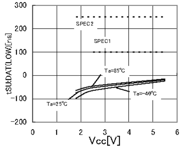
Figure 23. Input data setup time tSU:DAT(LOW)
