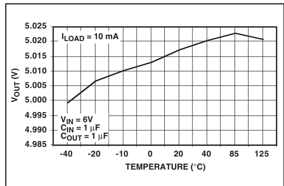
FIGURE 2-12: Output Voltage (5V) vs. Temperature ( I_{LOAD} = 10 mA ).
