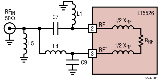
Figure 5. Schematic of Lumped Element Input Balun
