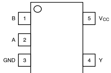
Pinout (Gates)
