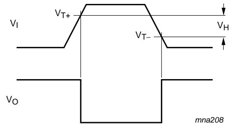
Fig 10. Definition of V_{T+} , V_{T-} and V_H
