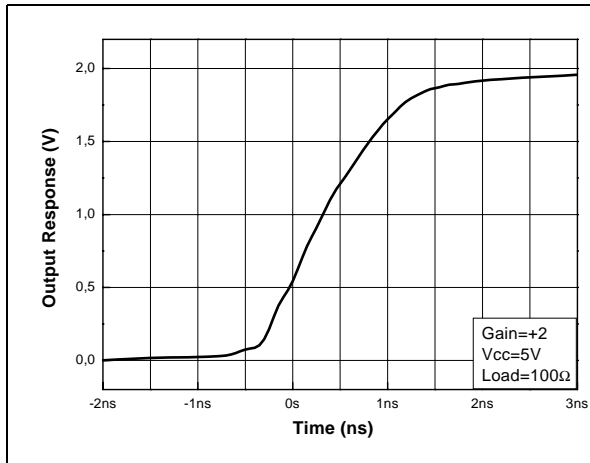
Figure 7. Slew rate
