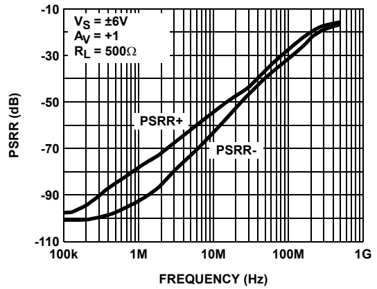
FIGURE 28. PSRR
