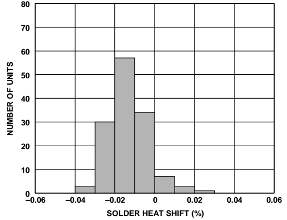
Figure 64. ADR4533 Solder Heat Resistance Shift (3 × Reflow)
