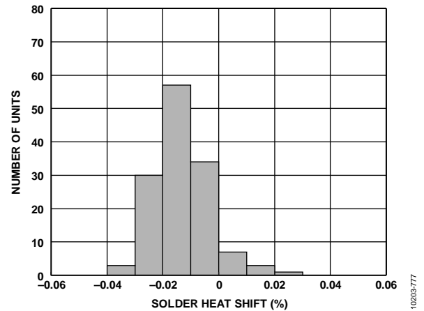
Figure 80. ADR4540 Solder Heat Resistance Shift (3 x Reflow)
