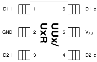
6-pin SC70
