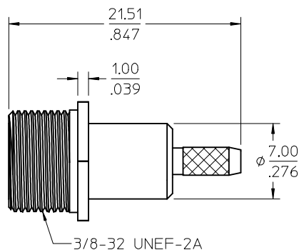
CABLE CONTACT
