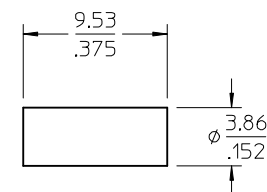
CRIMP TUBE
