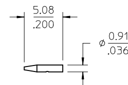
CABLE CONTACT
