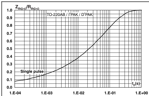
Figure 8. Relative thermal impedance junction to case versus pulse duration (TO-220AB / I²PAK / D²PAK)
