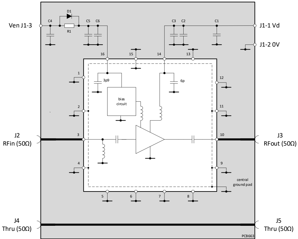
Figure 44: EV90G701 Schematic
