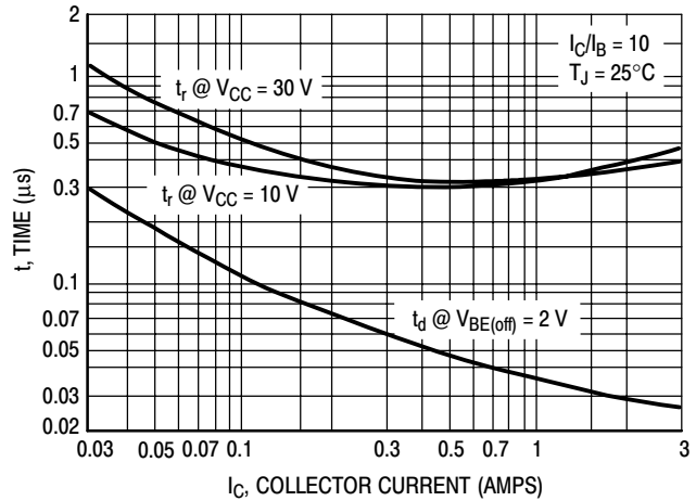
Figure 4. Turn-On Time
