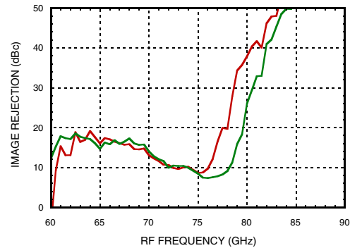
Image Rejection, USB vs. LO Drive
