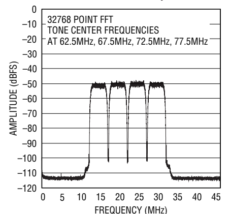
4-Tone WCDMA Waveform LT1993-4 Driving LTC2255 14-Bit ADC at 92.16Mps
