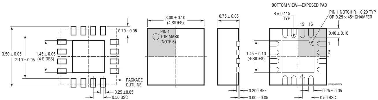
RECOMMENDED SOLDER PAD PITCH AND DIMENSIONS
