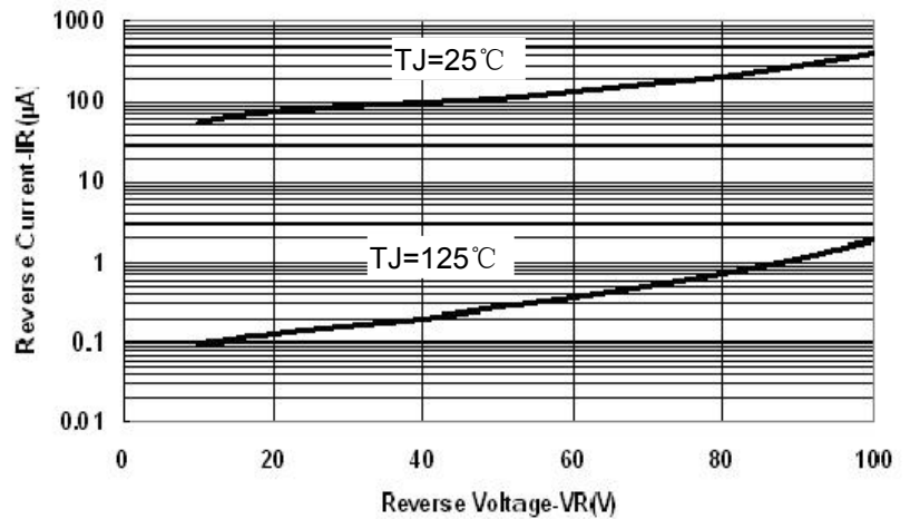
Fig.2-Typical Reverse Characteristics
