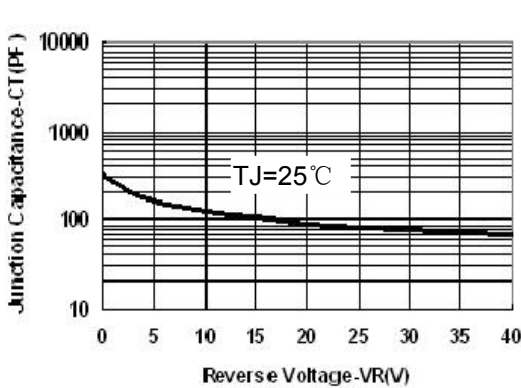
Fig.1-Typical Junction Capacitance
