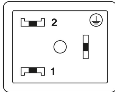
Valve connector pin assignment, type B
