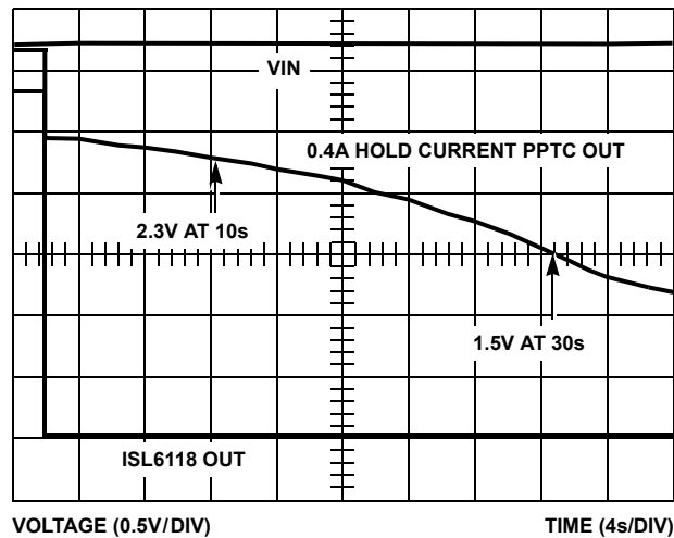
FIGURE 13. ISL6118 vs PPTC WITH EXTENDED 3.5Ω LOAD
