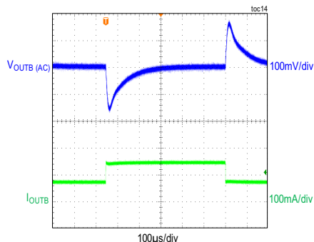
MAXM17720, MAXM17724 LOAD TRANSIENT RESPONSE
