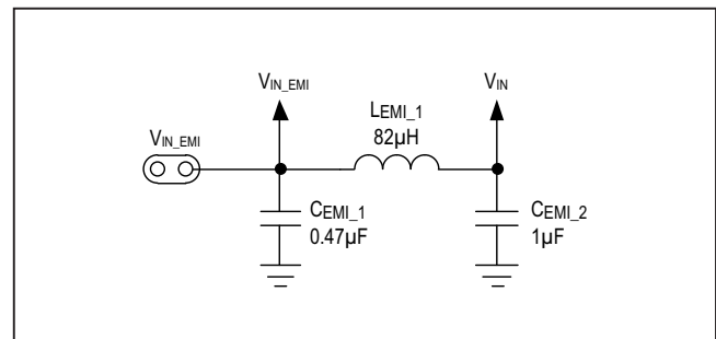
Figure 2. EMI Filter Components
