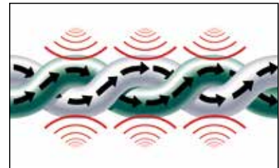
Illustration 2: Example of Bonded-Pair. As cable is stretched and pulled, pairs stay intact.
