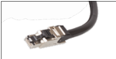
Metal Body Field-Installable Plug
