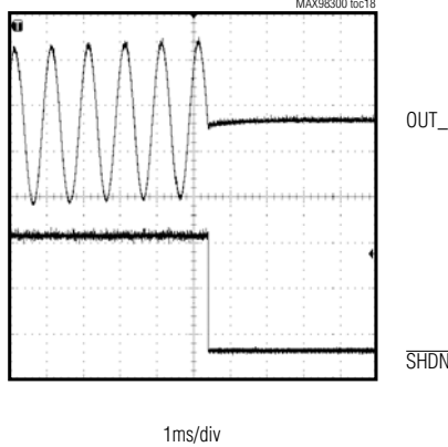
SHUTDOWN WAVEFORM
