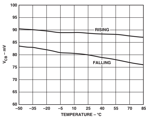
TPC 6. Circuit Breaker Current Limit Voltage, V_{CB} vs. Temperature
