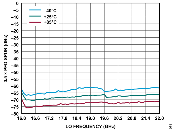
Figure 73. 0.5 \times PFD Spur vs. LO Frequency at Various Temperatures, Spur Referred to the Main I Channel and Q Channel Output Frequency
