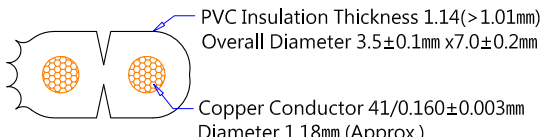
SPT-2 18AWGx2C 截面圖 (Wire Cross-Section)
