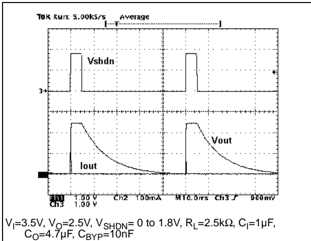
Figure 23. Start-up transient ( C_{\text{BYP}} = 10\text{ nF} )
