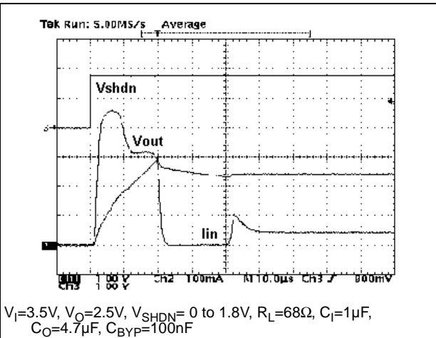
Figure 24. Start-up transient ( C_{\text{BYP}} = 100\text{ nF} )
