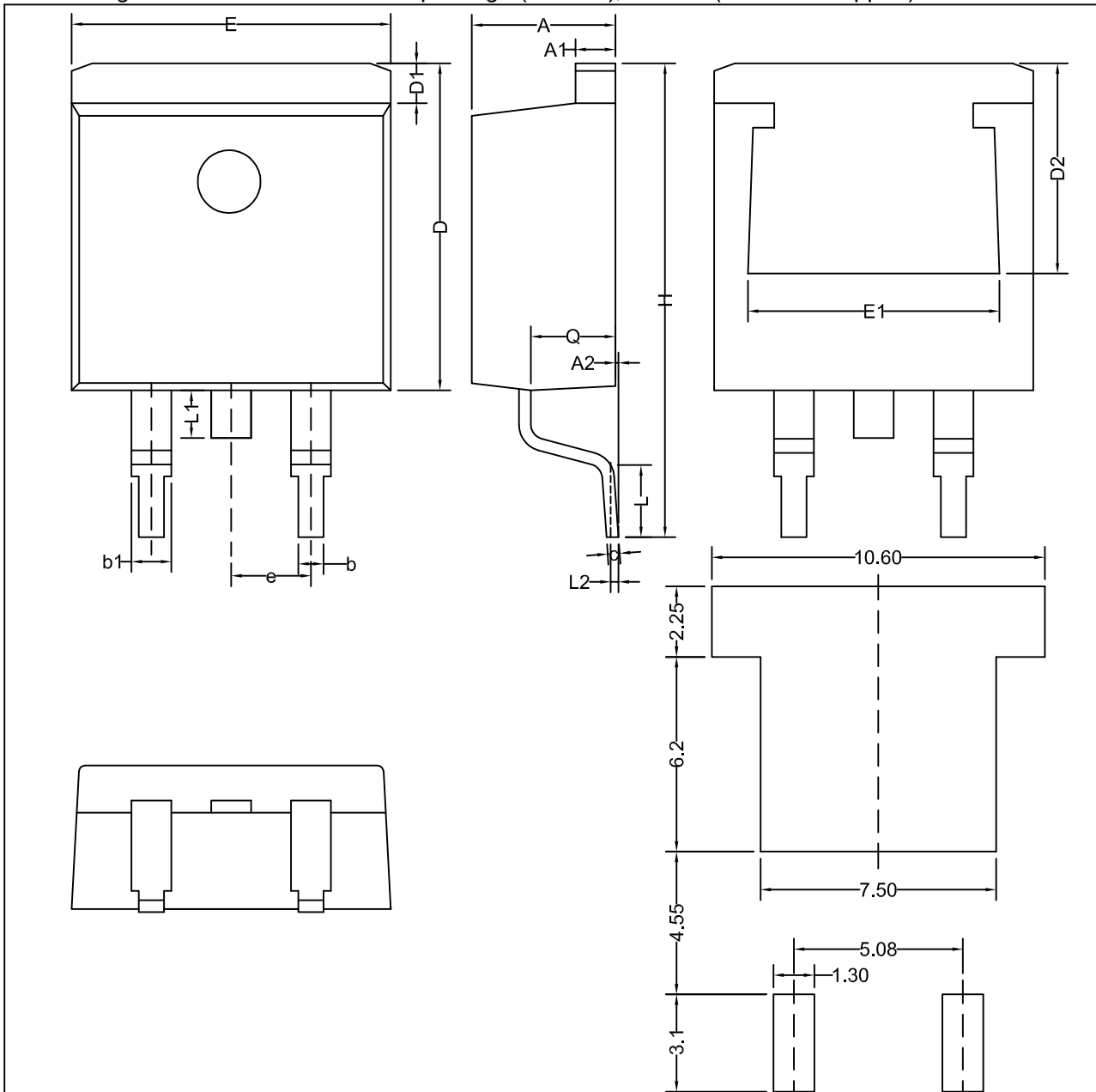
Recommended Footprint
