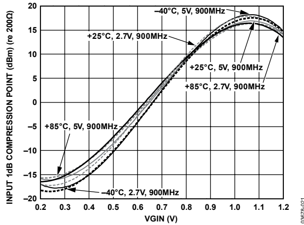
Figure 21. Input 1 dB Compression Point (IP1dB) vs. V_{GIN} , F_{IF} = 900\text{ MHz} , F_{BB} = 1\text{ MHz} , V_{POS} = 2.7\text{ V} , 5\text{ V} , Temperature = -40^\circ\text{C} , +25^\circ\text{C} , +85^\circ\text{C}
