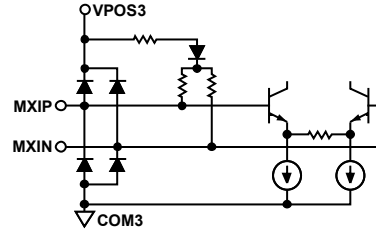
Figure 11. Circuit I
