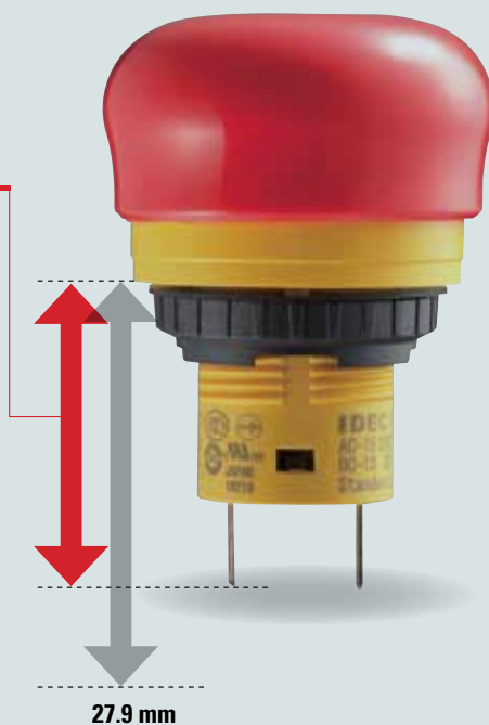
ø30 mm Button Unmarked
