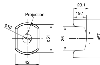
Switch Guard XA9Z-KG1
