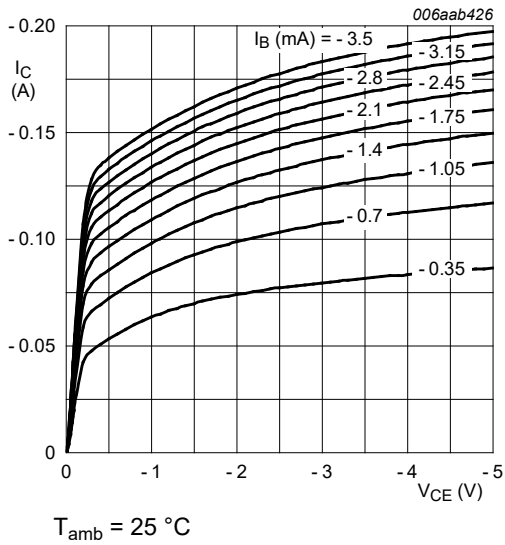
Fig. 7. PNP transistor: Collector current as a function of collector-emitter voltage; typical values
