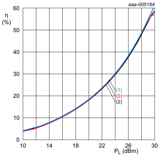
V_{SUP} = 3.6\text{ V} ; I_{CC(tot)} = 70\text{ mA} ; matched for ISM-434. (1) T_{amb} = -40^\circ\text{C} (2) T_{amb} = +25^\circ\text{C} (3) T_{amb} = +85^\circ\text{C}
