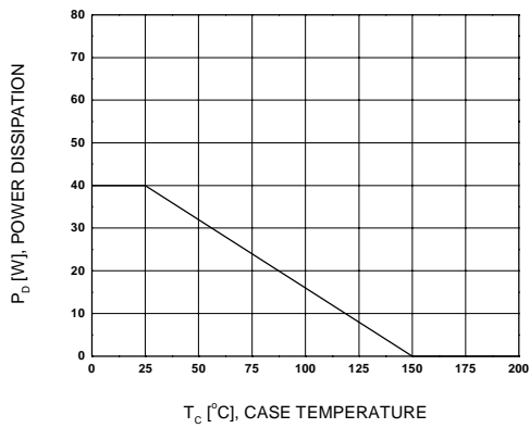
Figure 11. Power Derating
